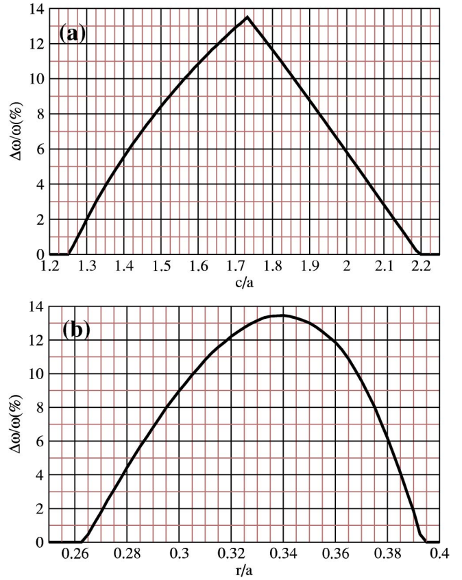
FIG. 6. T/[1,1] \oplus [-1,-1]^{(0,0.5)} family of photonic crystals. (a) Relative size of the full photonic band gap as a function of c for r=0.34a . (b) Relative size of the full photonic band gap as a function of r for c=1.73a . The dielectric constant of the background material is 11.9.
